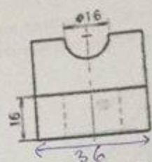
3D Object and its Orthographic Views
